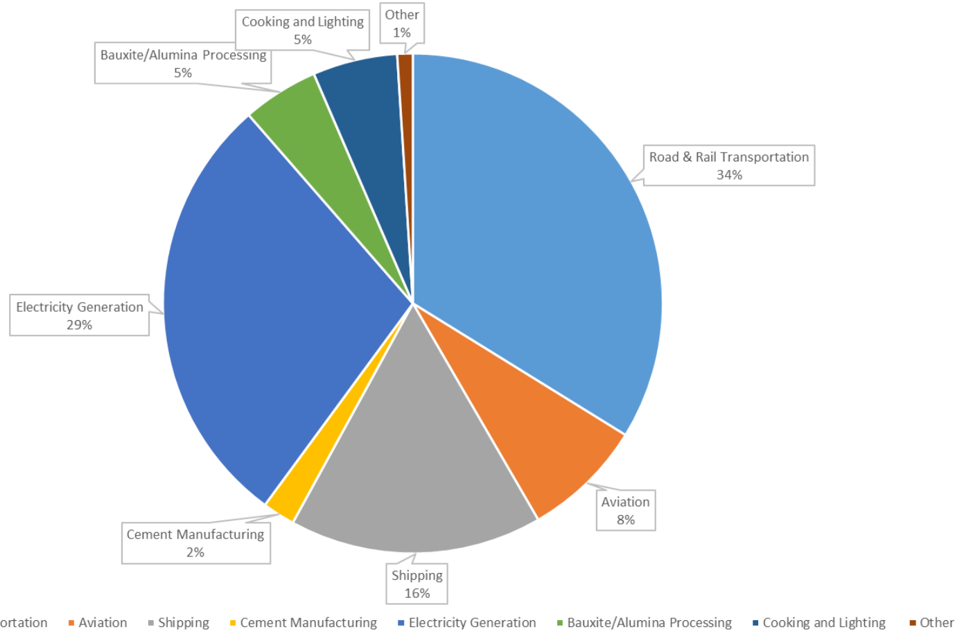
Petroleum Consumption by Activity 2023
